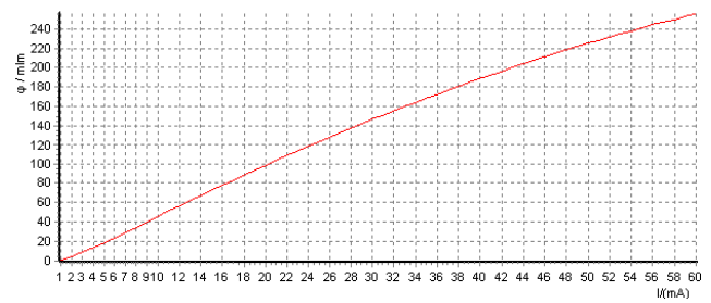
Current-Luminous flux Curve
